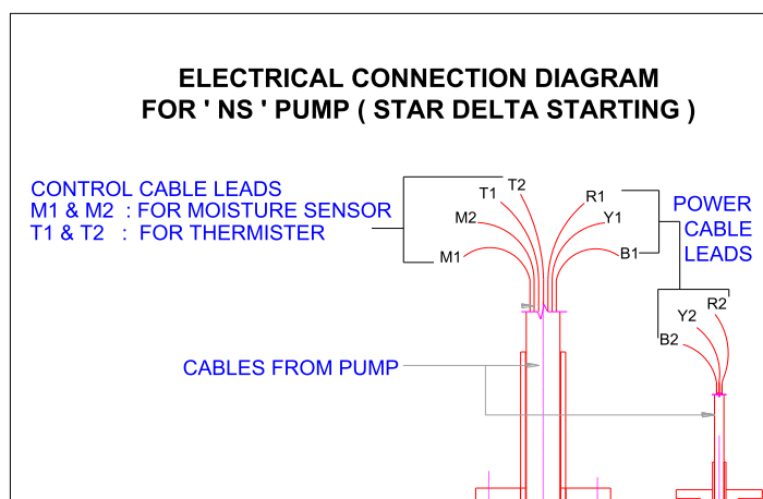
Figure (2): SDS-connection
