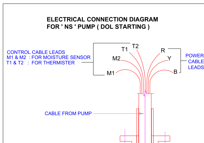
Figure (3): DOL-connection
